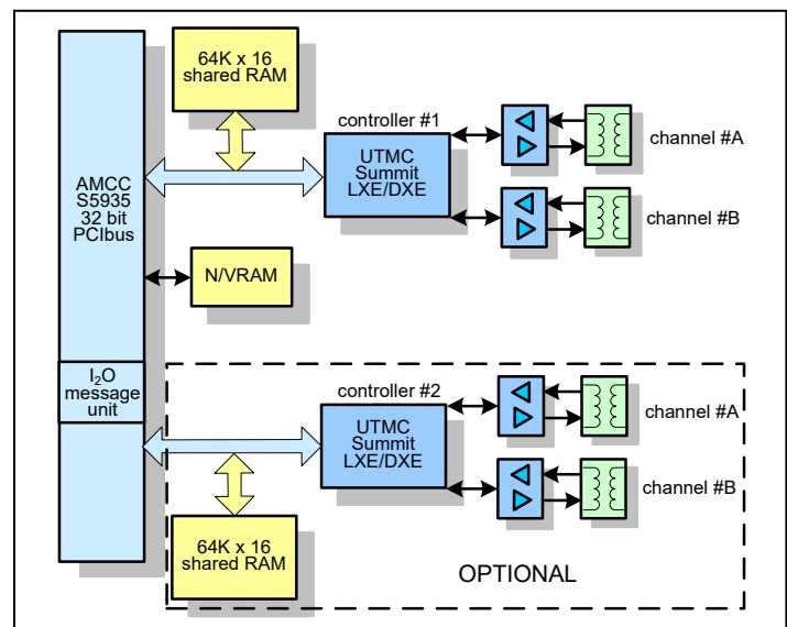
CPCI-1553-UTMC 2 shown
